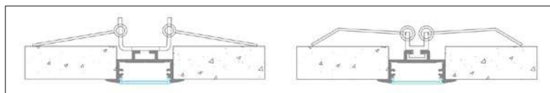
MONTAGGIO A INCASSO FLUSH-MOUNTED
