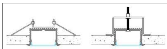
MONTAGGIO A INCASSO FLUSH-MOUNTED
