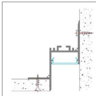
MONTAGGIO A PARETE WALL-MOUNTED
