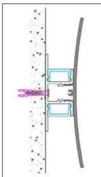
MONTAGGIO A PARETE WALL MOUNTED
