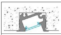
MONTAGGIO A INCASSO FLUSH-MOUNTED
