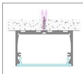
MONTAGGIO A PARETE WALL-MOUNTED
