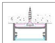
MONTAGGIO A PARETE CON CLIP WALL MOUNTED WITH CLIPS
