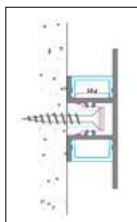
MONTAGGIO A PARETE WALL MOUNTED
