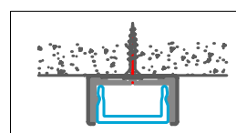
MONTAGGIO A PARETE CON CLIP WALL MOUNTED WITH CLIPS
