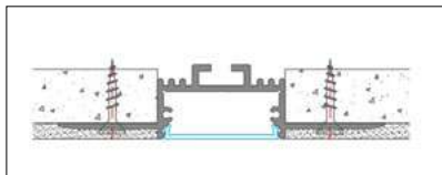
MONTAGGIO A INCASSO FLUSH-MOUNTED
