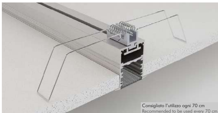
Staffa a molla con ali corte per fissaggio a cartongesso Spring bracket with short wings for fixing to plasterboard Cod. NM-008-B
