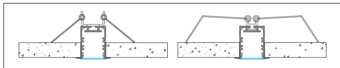
MONTAGGIO A INCASSO FLUSH-MOUNTED
