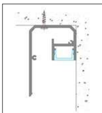
MONTAGGIO A PARETE WALL MOUNTED
