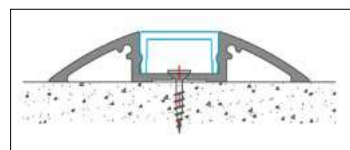
MONTAGGIO A PARETE WALL MOUNTED
