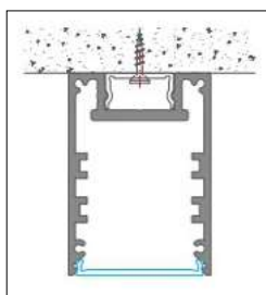
MONTAGGIO A PARETE WALL-MOUNTED
