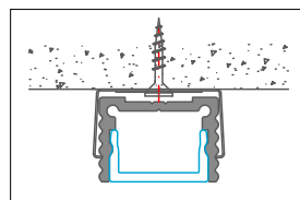
A PARETE CON GRAFFETTE WALL-MOUNTED WITH CLIP
